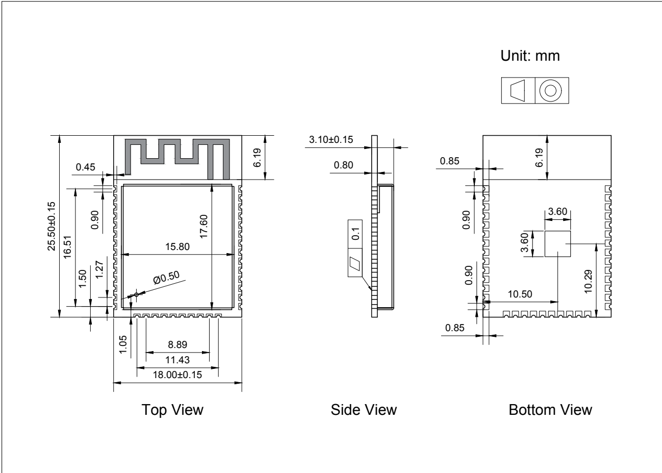
Figure 5: Physical Dimensions of ESP32-WROOM-32SE
